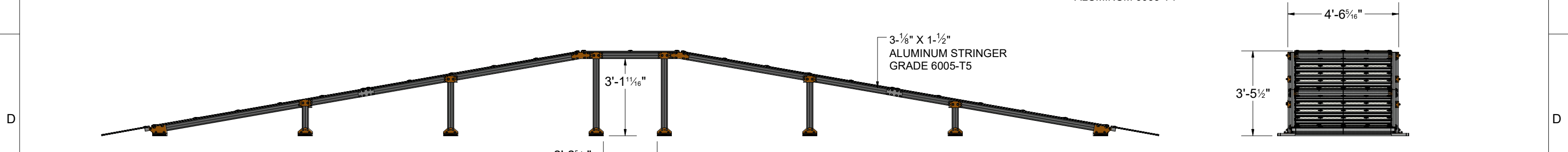
FRONT VIEW
